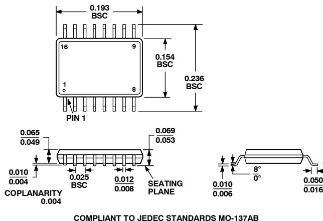
Figure 45. 16-Lead Shrink Small Outline Package [QSOP] (RQ-16) Dimensions shown in inches
