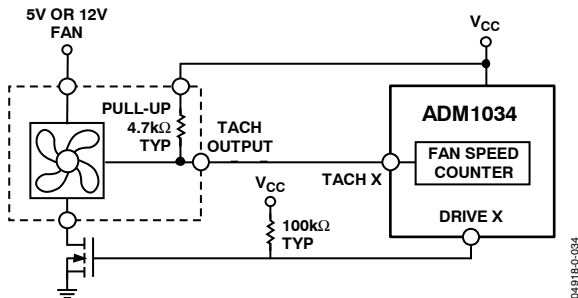
Figure 36. Fan with TACH Pull-Up to +V_{CC}
