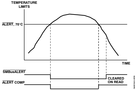
Figure 31. ALERT Comparator and SMBusALERT Outputs
