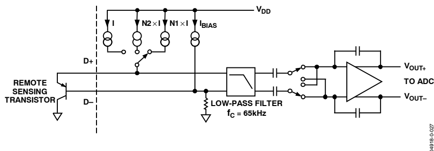
Figure 28. ADM1034 Signal Conditioning
