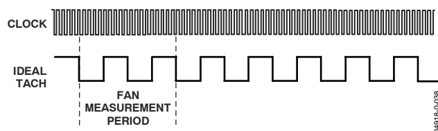
Figure 40. Fan Speed Measurement for a 4-Pole Fan
